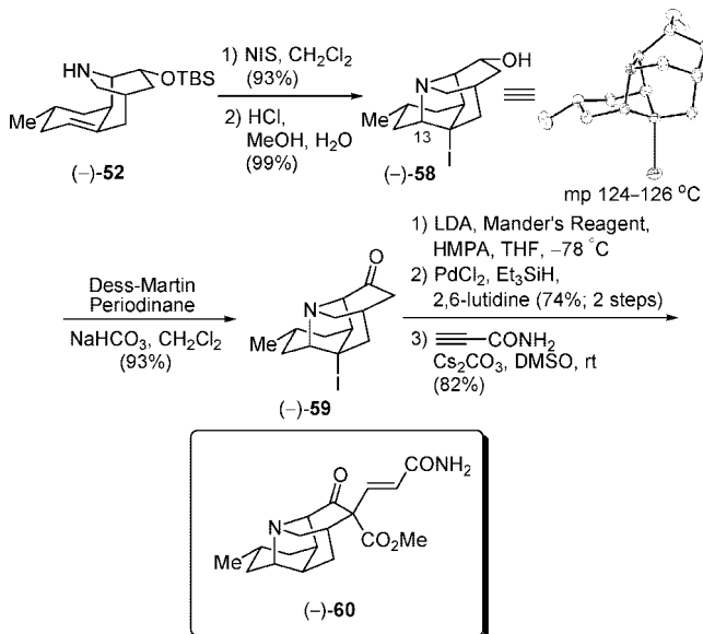
Scheme 14. Preparation of the Penultimate Intermediate for (+)-Lyconadin A ( 1 )
