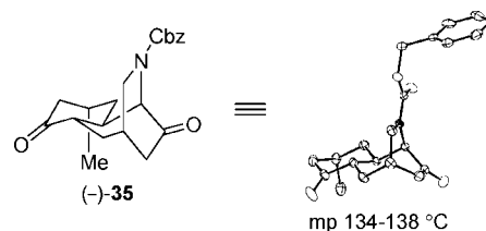
Figure 2. Structure of diketone (–)-35.
