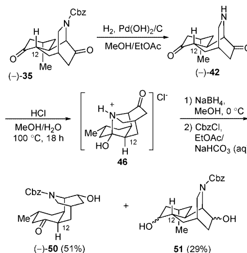
Scheme 11. Four-Step Sequence to Correct the C(12) Stereogenicity
