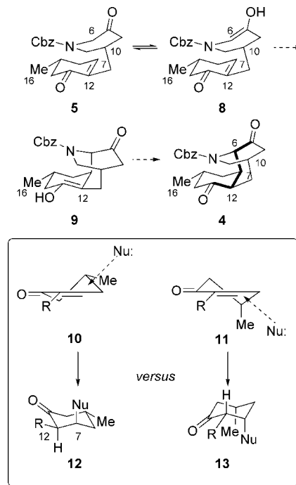
Scheme 2. Stereochemical Analysis of the Strategic Conjugate Addition
