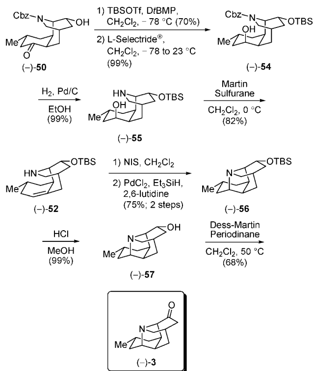
Scheme 13. Construction of the Tetracyclic Core of the Lyconadins
