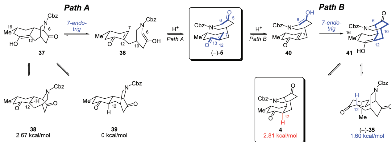
Scheme 8. Stereochemical Analysis of the Strategy-Level Conjugate Addition
