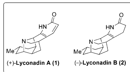
Figure 1. Structures of the alkaloids (+)-lyconadin A ( 1 ) and (–)-lyconadin B ( 2 ).
