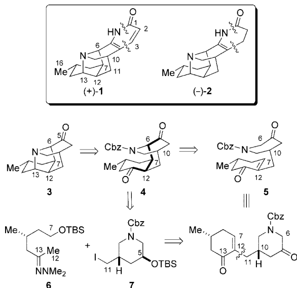
Scheme 1. Retrosynthetic Analysis of (+)-Lyconadin A ( 1 ) and (–)-Lyconadin B ( 2 )
