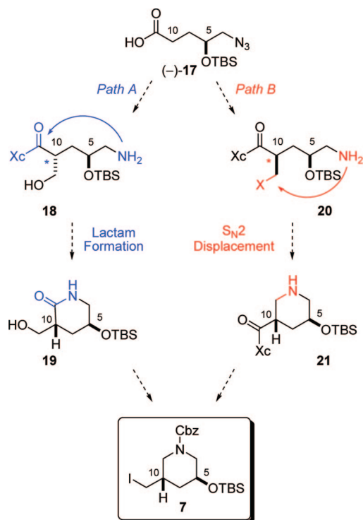
Scheme 4. Synthetic Strategies to Construct Iodide 7
