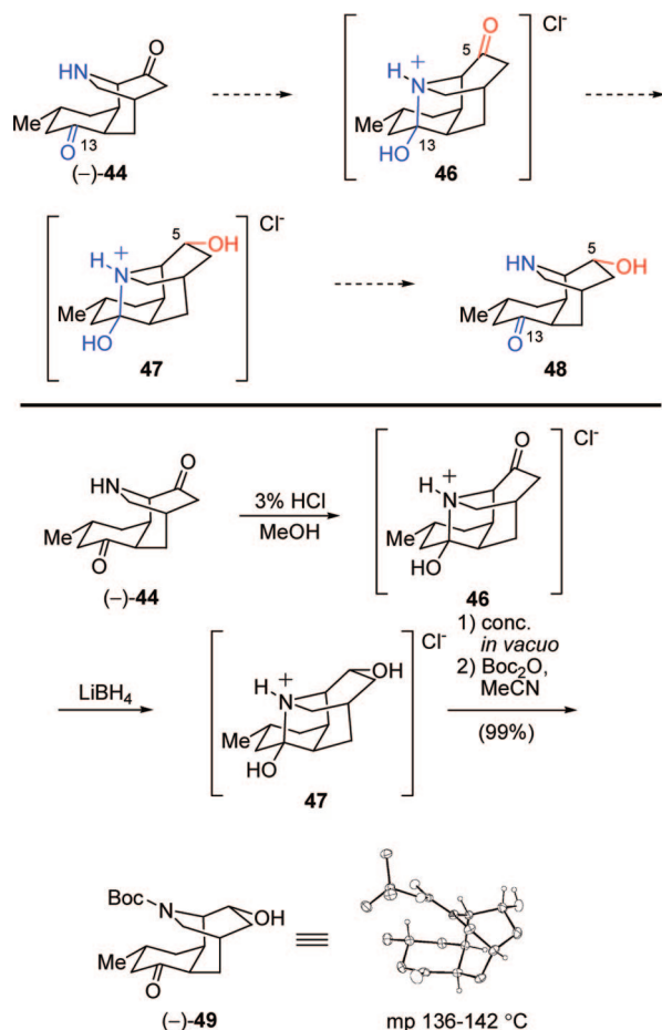
Scheme 10. Hemiaminal Mask for the C(13) Ketone
