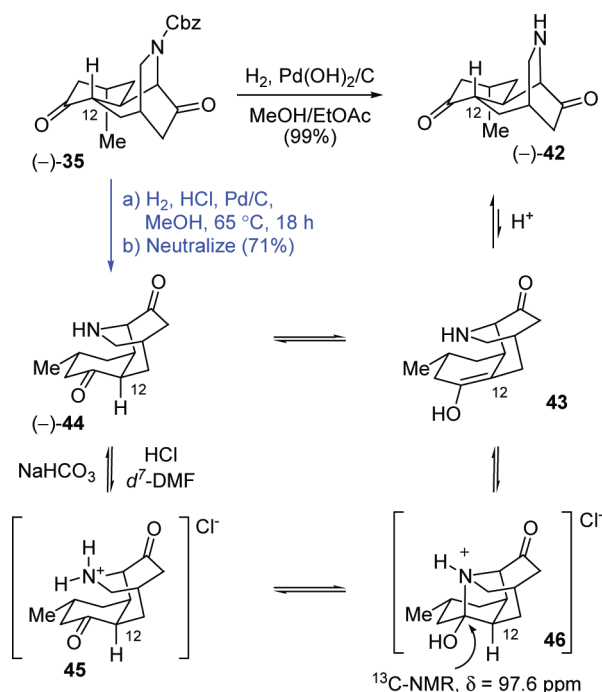
Scheme 9. Correction of the Stereogenicity at C(12)
