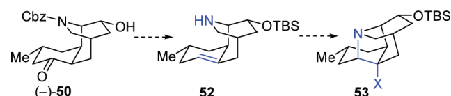
Scheme 12. Synthetic Strategy to Construct the Tetracyclic Core
