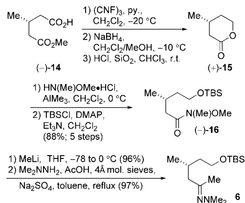
Scheme 3. Construction of Hydrazone 6
