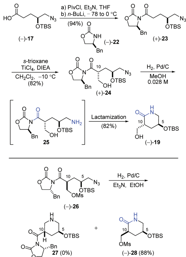
Scheme 5. Synthetic Approaches to Iodide 7
