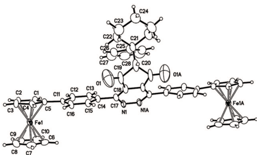
Figure 7. ORTEP drawing and stick representation of 8.
