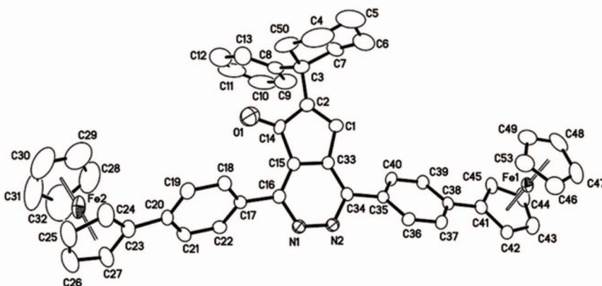
Figure 6. ORTEP drawing and stick representation of 7.
