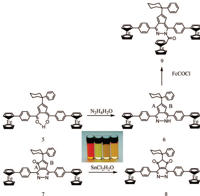
Scheme 2. Synthesis of Compounds 5 (red-orange), 6 (light yellow), 7 (brown), and 8 (light brown) in CH 2 Cl 2
