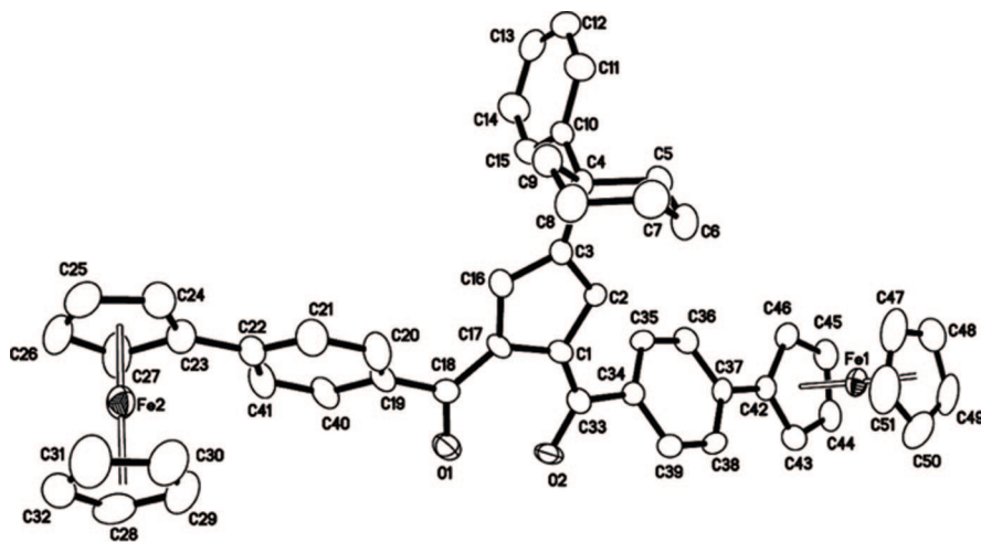
Figure 5. ORTEP drawing and stick representation of 5.
