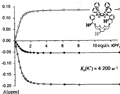
Fig. 2. ^1\text{H} -NMR Shifts observed for 1 on titration with \text{KPF}_6 in \text{CD}_3\text{CN} at 20^\circ . The dots represent the experimental data. Top: \text{O}-\text{CH}_2-\text{CH}_2-\text{O} signal at 3.56 ppm; middle: benzylic \text{CH}_2 signal at 3.8 ppm; bottom: aromatic H signal at 6.78 ppm. The solid lines are the calculated curves for K_a(\text{K}^+) = 4200 \text{ M}^{-1} .
