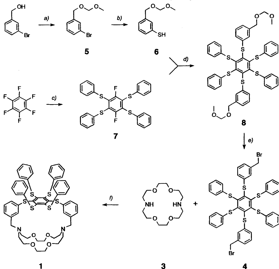
Scheme 2. Synthesis of the Macrobicyclic Ligand 1
