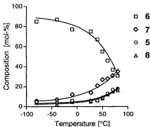
Figure. Equilibrium composition of the mixture 5–8 in \text{CDCl}_3 solution as a function of the temperature (ratios determined by ^1\text{H-NMR} )
