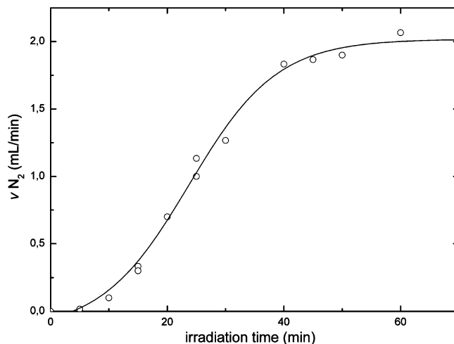
Figure 9. Rate of \text{N}_2 formation versus irradiation time (at 90 °C).
