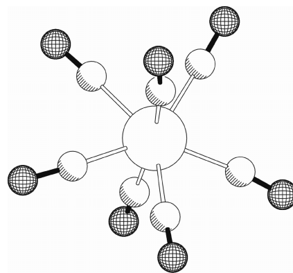
Figure 4. Structure of the [\text{Mo}(\text{CN})_7]^{5-} ion in 1 .
