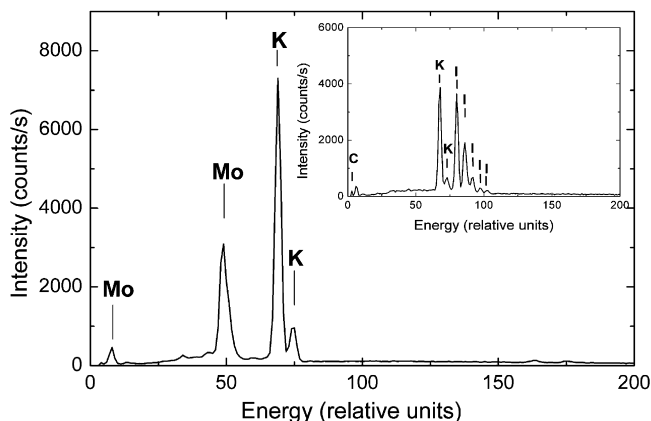
Figure 2. EDS spectrum of \text{K}_5[\text{Mo}(\text{CN})_7] \cdot \text{N}_2\text{H}_4 ( 1 ). In the upper right corner, the EDS spectrum of KI is presented for comparison.
