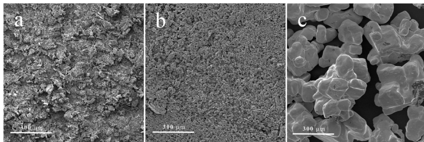
Figure 1. Scanning electron microscope photographs of (a) KI, (b) \text{K}_5[\text{Mo}(\text{CN})_7] \cdot \text{N}_2\text{H}_4 , and (c) \text{K}_4[\text{Mo}(\text{CN})_8] \cdot 2\text{H}_2\text{O} .
