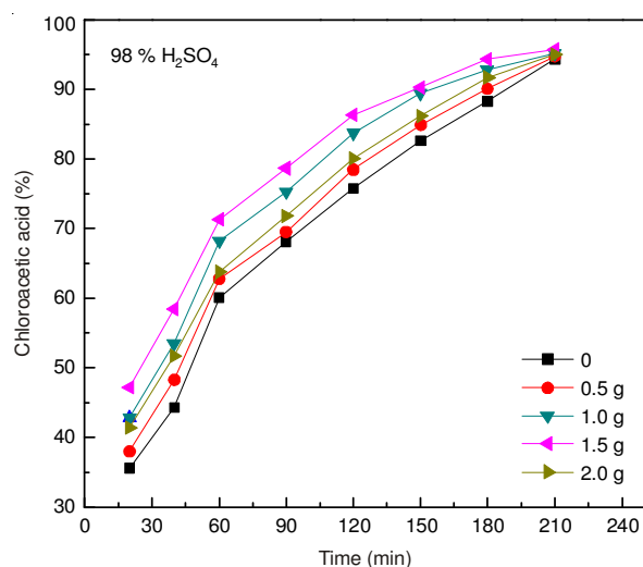
Fig. 4. Influence of cocatalyst 98 % \text{H}_2\text{SO}_4 on the production of chloroacetic acid. The different amounts of \text{H}_2\text{SO}_4 added in mixture are 0, 0.5, 1, 1.5 and 2 g, respectively
