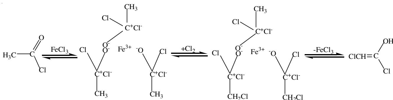
Scheme-I: Cocatalytic mechanism of \text{FeCl}_3 on chlorination reaction
