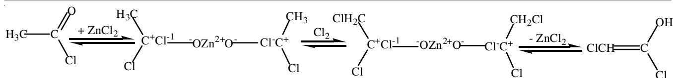
Scheme-II: Cocatalytic mechanism of \text{ZnCl}_2 on chlorination reaction
