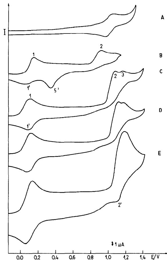
Fig. 5. Cyclic voltammograms of thiatetra( p -tolyl)porphyrin (STpTP) and its Cu(II) complexes. A, 1.3 mM STpTP in 0.1 M TBAP– \text{C}_2\text{H}_4\text{Cl}_2 , \nu = 50 \text{ mV s}^{-1} ; B, 0.7 mM \text{Cu(STpTP)HCO}_3 in 0.1 M TBAP– \text{CH}_3\text{CN} , \nu = 100 \text{ mV s}^{-1} ; C, D, E, 1.3 mM \text{Cu(STpTP)HCO}_3 in 0.1 M TBAP– \text{C}_2\text{H}_4\text{Cl}_2 , \nu = 100 \text{ mV s}^{-1} , \nu = 150 \text{ mV s}^{-1} , \nu = 400 \text{ mV s}^{-1} , respectively.
