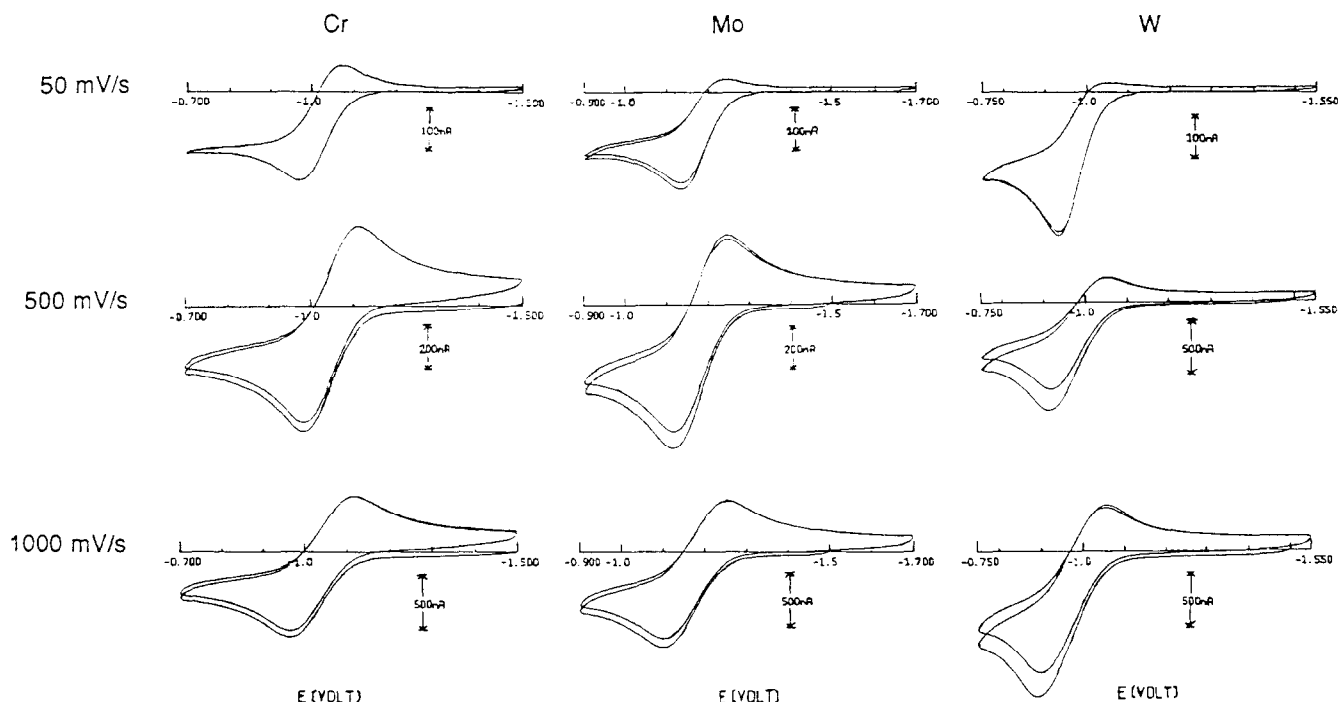
Fig. 1. Cyclic voltammograms of [\text{M}_2(\text{CO})_{10}]^{2-} in THF at various sweep rates.
