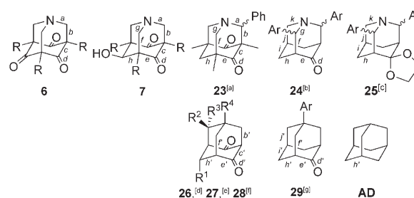
Figure 5. Atom labeling scheme for the bond length data presented in Table 2. R = \text{CH}_2\text{CO}_2i\text{Pr} , R^1 – R^4 = various substituents, Ph = phenyl, Ar = p -nitrophenyl ( 24 ) or p -chlorophenyl ( 25 ), AD = various adamantanes. Reference (CSD code): [a] ref. [24] (KOLSIN); [b] ref. [25] (OCAYEW); [c] ref. [26] (EJIQUJ); [d] ref. [28] (DESVIG); [e] ref. [29] (LIXFIH); [f] ref. [29] (LIXFUT); [g] ref. [30] (FITPED).
