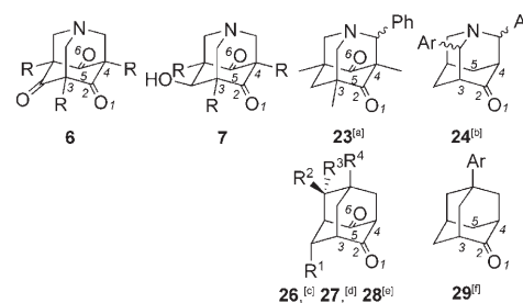
Figure 6. Atom labeling scheme for the bond angle data presented in Table 3. R = \text{CH}_2\text{CO}_2i\text{Pr} , R^1 – R^4 = various substituents, Ph = phenyl, Ar = p -nitrophenyl. Reference (CSD code): [a] ref. [24] (KOLSIN); [b] ref. [25] (OCAYEW); [c] ref. [28] (DESVIG); [d] ref. [29] (LIXFIH); [e] ref. [29] (LIXFUT); [f] ref. [30] (FITPED).
