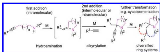
Scheme 1. Cyclization-Triggered Alkynylation
