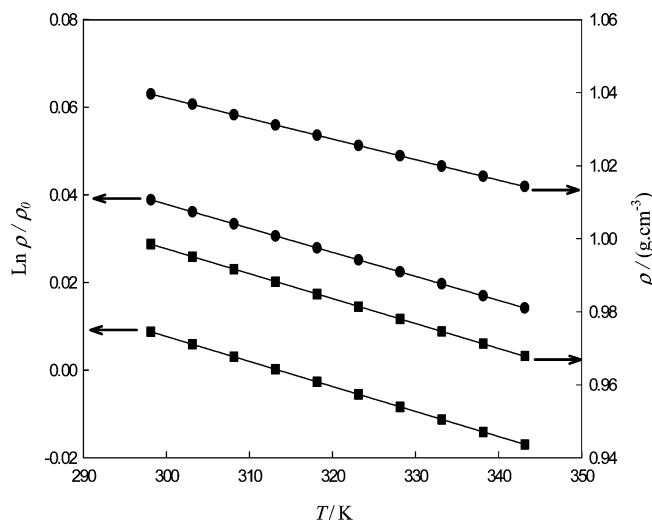
Figure 1. Experimental values of \ln \rho/\rho_0 and \rho for \bullet , [C 6 mim][Cl]; and \blacksquare , [C 8 mim][Cl] plotted against temperature and fitted lines. For [C 6 mim][Cl]: \ln \rho/\rho_0 = 0.2024 - 5 \cdot 10^{-4} T/K and \rho/\text{g}\cdot\text{cm}^{-3} = 1.2075 - 6 \cdot 10^{-4} T/K . For [C 8 mim][Cl]: \ln \rho/\rho_0 = 0.2179 - 6 \cdot 10^{-4} T/K and \rho/\text{g}\cdot\text{cm}^{-3} = 1.1783 - 6 \cdot 10^{-4} T/K .
