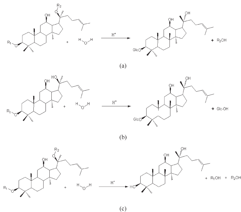
Figure 7. The generation of rare ginsenosides Rg_3 (a), Rh_2 (b) and aglycon (c) in neutral solution.
