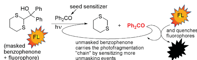
Scheme 1 General concept for the massive amplified unmasking of benzophenone resulting in fluorescence quenching (see text).
