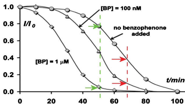
Fig. 1 Quenching of quaterphenyl as a result of benzophenone (BP) amplification ( y -axis is the normalized emission at 360 nm).
