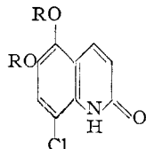
XXX, R = H XXXI, R = CH 3 CO
