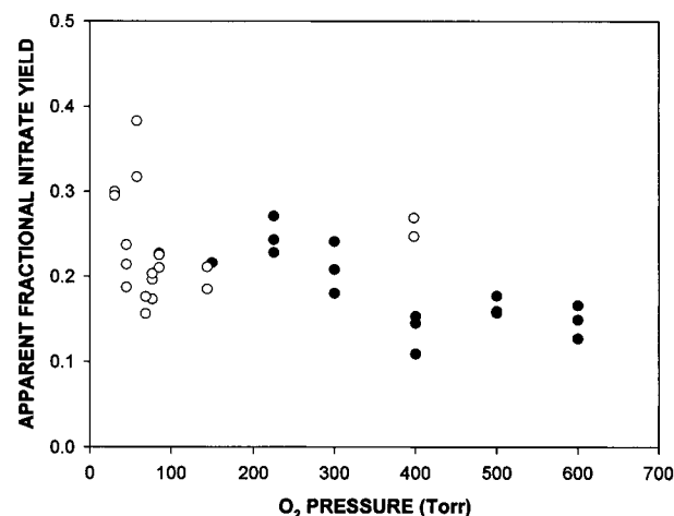
Figure 1. Plot of the apparent nitrate yield as a function of \text{O}_2 partial pressure in the photolysis of \text{Cl}_2 /cyclohexane/ \text{NO}/\text{O}_2/\text{N}_2 mixtures at 700 Torr total pressure. Open circles, 273 K; Filled circles, 296 K.
