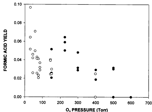
Figure 4. Formic acid yield as a function of \text{O}_2 partial pressure in the photolysis of \text{Cl}_2/\text{cyclohexane}/\text{NO}/\text{O}_2/\text{N}_2 mixtures at 700 Torr total pressure. Filled circles, 296 K; Open circles, 273 K.
