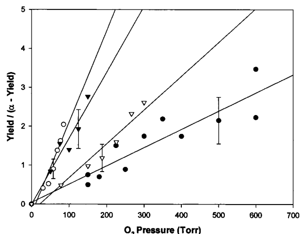
Figure 2. Plots of \text{Yield}/(\alpha - \text{Yield}) vs \text{O}_2 partial pressure in the photolysis of \text{Cl}_2/\text{cyclohexane}/\text{NO}/\text{O}_2/\text{N}_2 mixtures at 700 Torr total pressure, where Yield refers to the yield of cyclohexanone and (1 - \alpha) is the cyclohexyl nitrate yield (see text for details). Filled circles, 296 K; Open triangles, 288 K; Filled triangles, 280 K; Open circles, 273 K.
