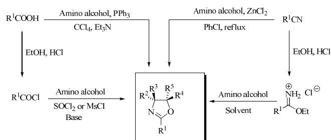
Scheme 1: Common routes for the construction of 2-oxazolines.
