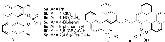
Figure 1. Catalysts evaluated in this study.
