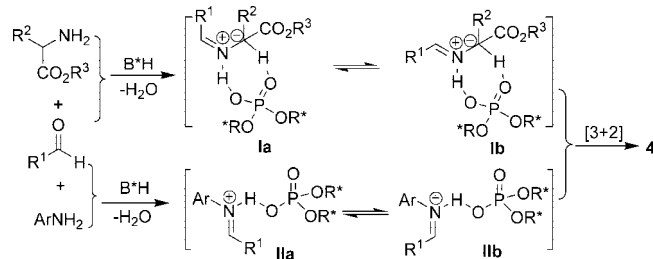
Scheme 1. Proposed Phosphoric Acid Catalyzed 1,3-Dipolar Cycloaddition of Imines with Azomethine Ylides
