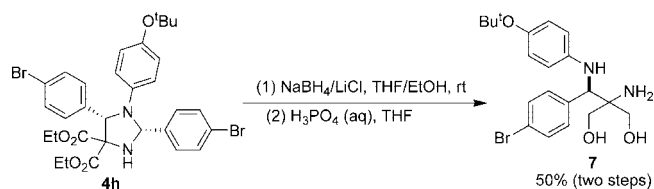
Scheme 2. Synthetic Application of Imidazolidines
