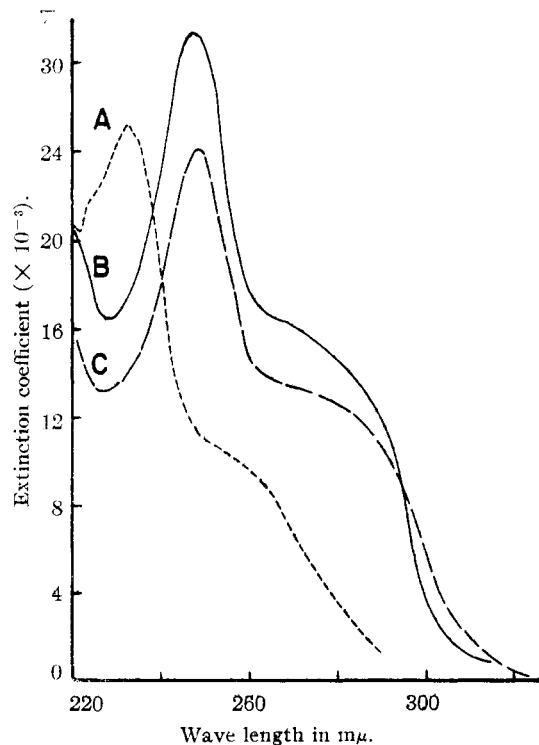
Fig. 4.—Ultraviolet absorption spectra of o -terphenyl, A; 4',4''-dimethoxy- o -terphenyl, B; 4',4''-dihydroxy- o -terphenyl, C.
