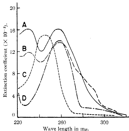
Fig. 1.—Ultraviolet absorption spectra of 2,3-bis-( p -methoxyphenyl)-cyclohexene, A; 2,3-bis-( p -hydroxyphenyl)-cyclohexene, B; styrene, C; anethole, D.
