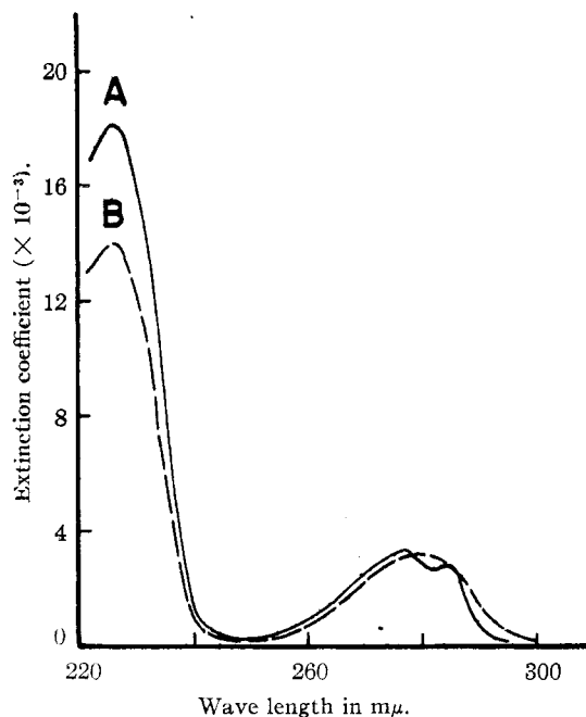
Fig. 3.—Ultraviolet absorption spectra of 1,2-bis-( p -methoxyphenyl)-cyclohexene, A; 1,2-bis-( p -hydroxyphenyl)-cyclohexene, B.
