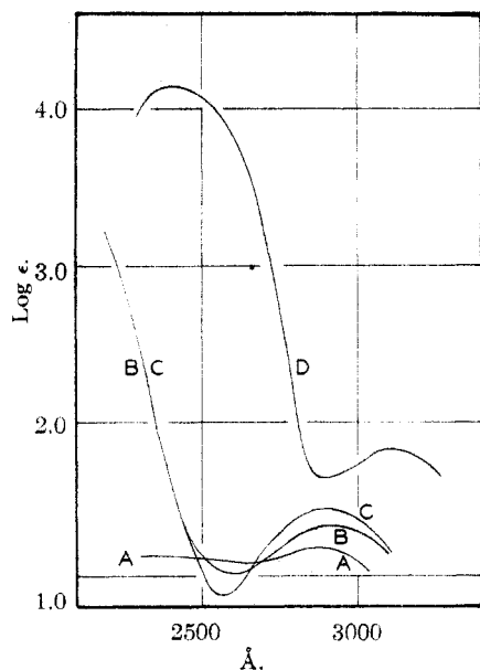
Fig. 2.—Absorption spectra of 3-cholestanone (VIII), A, carone (XI), B, i -cholestenone (X), C, and \Delta^3 -3-cholestenone, D. D is from H. Mohler, Helv. Chim. Acta , 20, 289 (1937).
