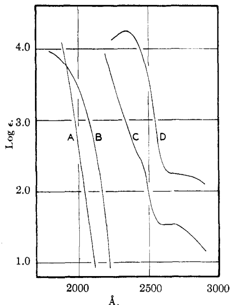
Fig. 1.—Absorption spectra of diallyl, A, trimethylethylene, B, \Delta^6 - i -cholestadiene (I), C, and cholestadiene, D. A and B from G. Scheibe and R. Pummerer, Ber. , 60 , 2163 (1927), and D from E. L. Skau and W. Bergmann, J. Org. Chem. , 3 , 166 (1938).
