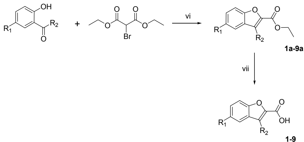
Scheme 2. vi) anhydrous K_2CO_3 , acetone, reflux; vii) 2N NaOH, THF
