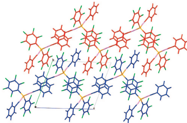
Figure 9. Illustrating the off \text{Ph}_\text{H} \cdots \text{Ph}_\text{H} and \text{Ph}_\text{F} \cdots \text{Ph}_\text{F} pairing interactions, connecting adjacent sheets, in 1 , viewed along the a axis. The carbon atoms are colored blue and red to indicate different sheets.
