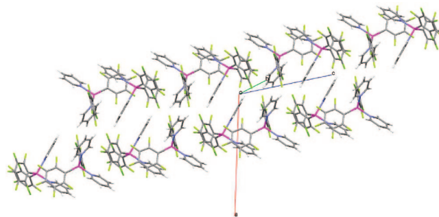
Figure 5. Packing in compound 4 .
