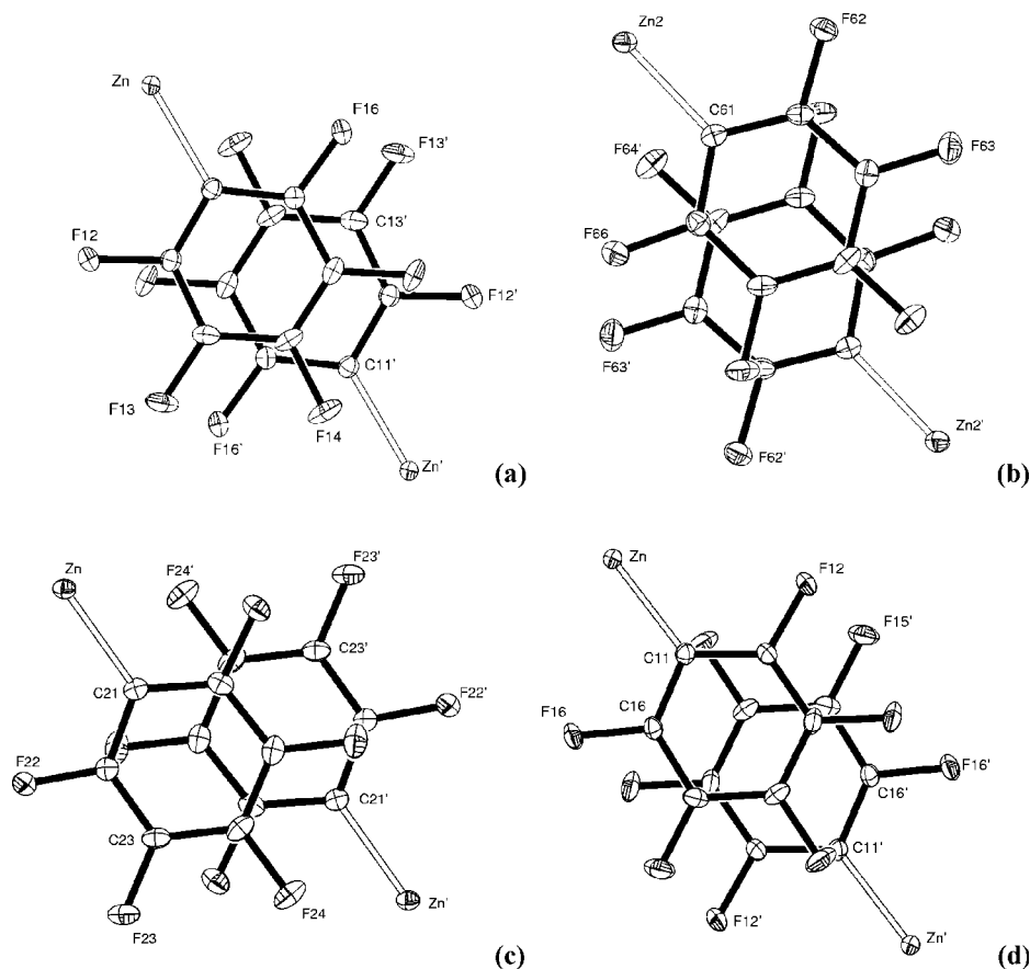
Figure 16. Selected projections of overlapping \text{Ph}_\text{F} \cdots \text{Ph}_\text{F} rings (the upper ring is in the plane of the page) in 1 (a), 2 (b), and 3 (c, d). Displacement ellipsoids are drawn at 30% probability.
