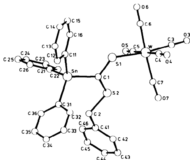
Fig. 2. Molecular structure of (\text{C}_6\text{H}_5)_3\text{SnCS}_2\text{CH}_2\text{C}_6\text{H}_5 \cdot \text{W}(\text{CO})_5 ( 2b ).
