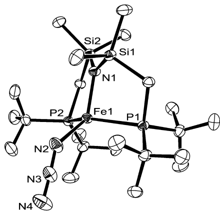
Figure 3. ORTEP view (50% probabilities) of the non-hydrogen atoms of (\text{PNP})\text{Fe}(\text{N}_3) . Unlabeled atoms are carbon. Selected structural parameters: \text{Fe1}-\text{N2} = 1.9613(14) Å, \text{Fe1}-\text{N1} = 1.9691(12) Å, \text{Fe1}-\text{P2} = 2.4878(4) Å, \text{Fe1}-\text{P1} = 2.5503(4) Å, \text{N2}-\text{N3} = 1.191(2) Å, \text{N3}-\text{N4} = 1.151(2) Å, \text{N2}-\text{Fe1}-\text{N1} = 131.00(6)^\circ , \text{N2}-\text{Fe1}-\text{P2} = 106.28(5)^\circ , \text{N1}-\text{Fe1}-\text{P2} = 94.16(4)^\circ , \text{N2}-\text{Fe1}-\text{P1} = 103.66(5)^\circ , \text{N1}-\text{Fe1}-\text{P1} = 136.333(15)^\circ , \text{N3}-\text{N2}-\text{Fe1} = 137.46(14)^\circ , \text{N4}-\text{N3}-\text{N2} = 175.9(2)^\circ .
