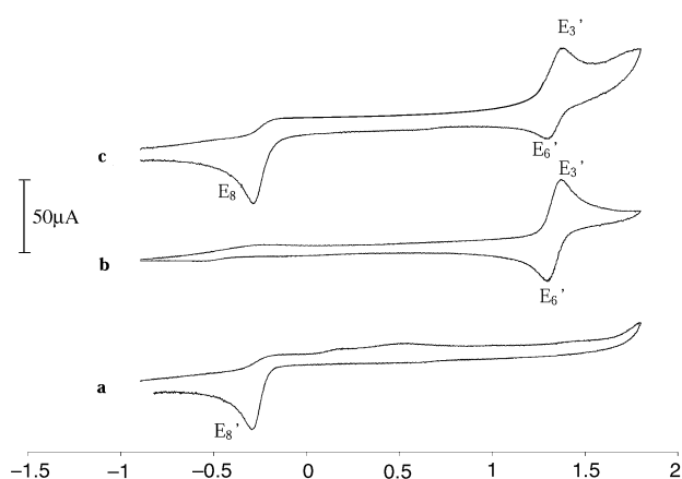
Fig. 10 Voltamperograms corresponding to compound 1 (curve a), methylaquocobaloxime (curve b) and a mixture of the compounds in 1 : 1 ratio (curve c) in acetonitrile as a solvent.
