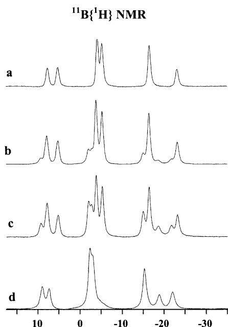
Fig. 1 ^{11}\text{B}\{^1\text{H}\} NMR spectra of the reaction of compound 1 with \text{THF} \rightarrow \text{BH}_3 at different 1 : \text{THF} \rightarrow \text{BH}_3 ratios: (a) 1 : 0, (b) 1 : 0.25, (c) 1 : 0.50, (d) 1 : 1.
