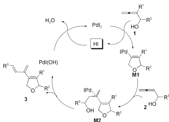
Scheme 4. Possible mechanism for the dimeric coupling–cyclization reaction of 1 with 2 .
