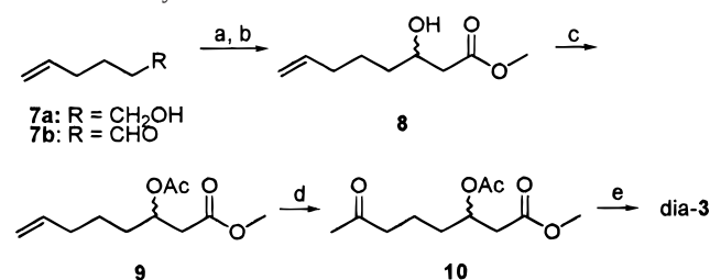
Scheme 1. Synthesis of Dia-3 a
