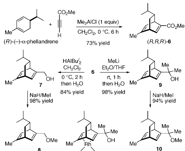
Scheme 1. Synthesis of Chiral Dienes
