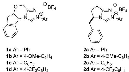
Figure 1. Chiral triazolium salts.
