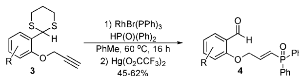
Scheme 1. Rhodium-Catalyzed Hydrophosphinylation
