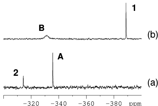
Figure 2. ^{15}\text{N}\{^1\text{H}\} NMR spectra (THF- d_8 , 298 K, 41 MHz, referenced to nitromethane) of 1 (a) after the addition of KOBu' and (b) after the addition of 2,6-lutidinium triflate (A = \text{NH}_2\text{NH}_2 ; B = \text{NH}_3\text{NH}_3^{2+} ).
