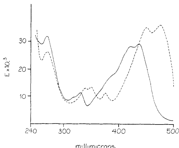
Fig. 3.—Ultraviolet spectrum of synthetic (±)-amide 39: in acidified methanol, —; in 0.001 N methanolic NaOH after standing 10 min., -----.
