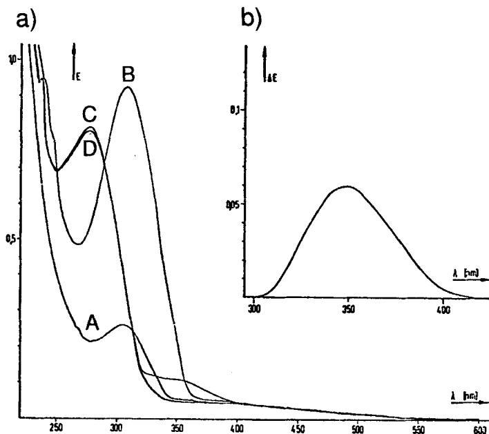
Fig. 9. Electronic absorption spectra of rac-1 in EPA before and after irradiation at low temperature with 365-nm light. a) Before irradiation at -185^\circ (A); after irradiation at -185^\circ for 150 min (B) after warming up to -163^\circ during 210 min in the dark (C); after warming up to r.t. and cooling down to -163^\circ (D); b) difference spectrum by subtraction of D from C (see Exper. 1.3.2.1.2).
