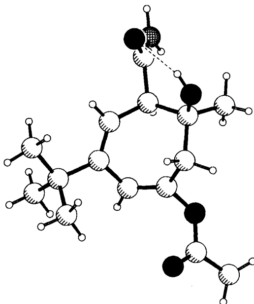
Fig. 19. Representation of single-crystal X-ray structure of rac -38a
