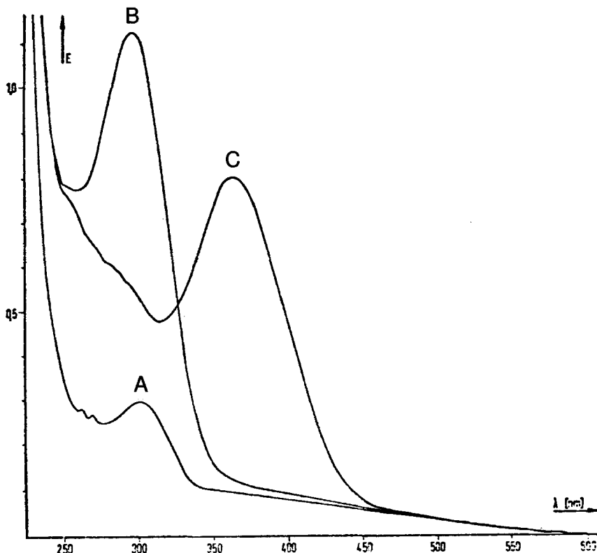
Fig. 11. Electronic absorption spectra of rac -1 and related transients in MCI. A: rac -1 at -185^{\circ} ; B: ketene transient obtained after irradiation with 365 nm-light at -152^{\circ} ; C: zwitterion transient formed after addition of DABCO at -150^{\circ} (see Exper. 1.3.2.2.1).
