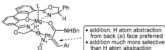
FIGURE 2. Substrate–Lewis acid binding model.
