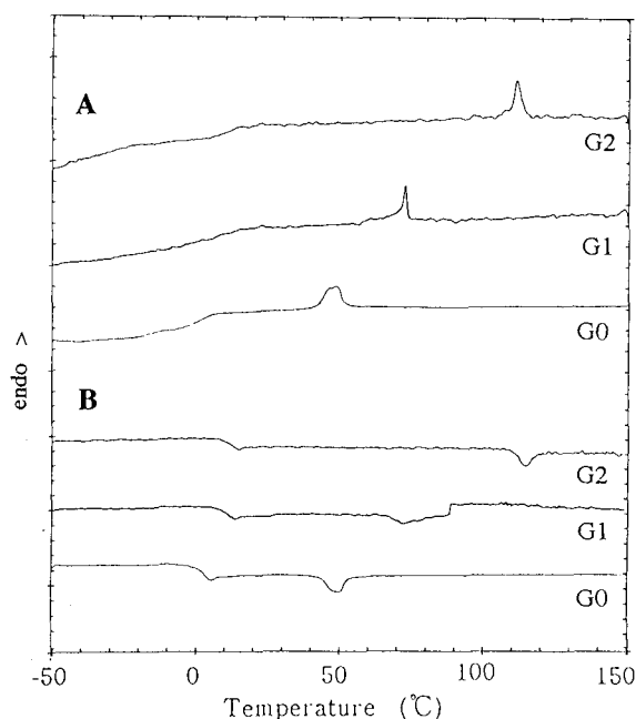
Figure 2. The DSC traces of Gn-mesogen ( n=0, 1, 2 ), A; cooling, B; 2nd heating.
