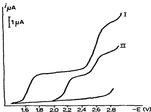
Fig. 1. Polarographic reduction waves of coordinated and non-coordinated acetophenone: (I) \text{C}_6\text{H}_5\text{COCH}_3\text{Cr(CO)}_3 ; (II) \text{C}_6\text{H}_5\text{COCH}_3 ; \text{CH}_3\text{CN} , 0.1 N (\text{C}_2\text{H}_5)_4\text{NClO}_4 .
