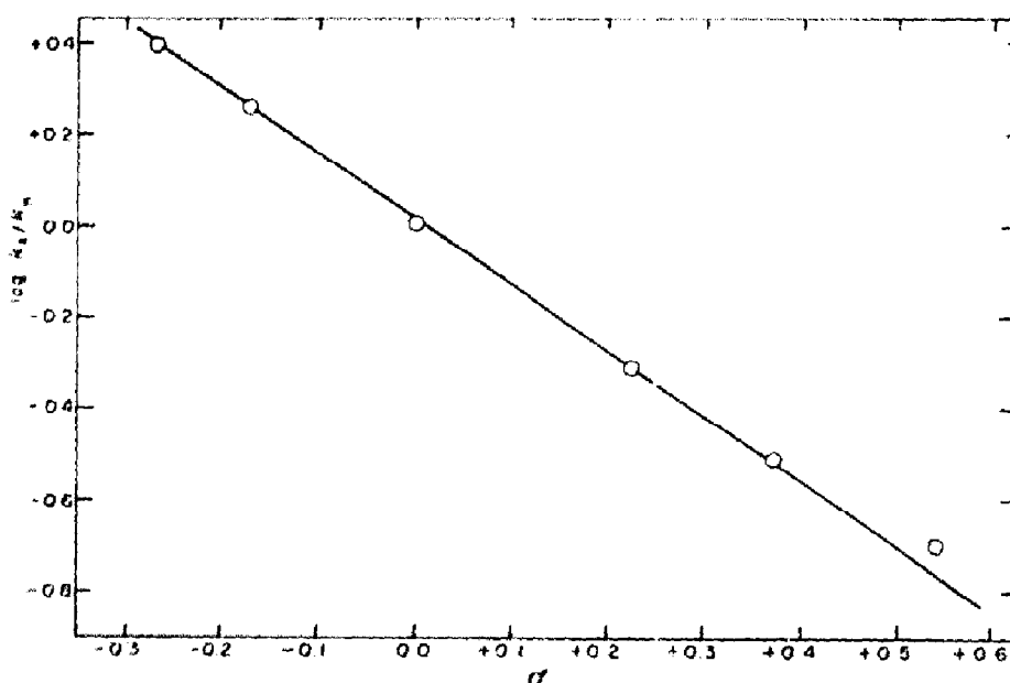
Fig. 1. Correlation of rates of ozone reaction with aryldimethylsilanes.
