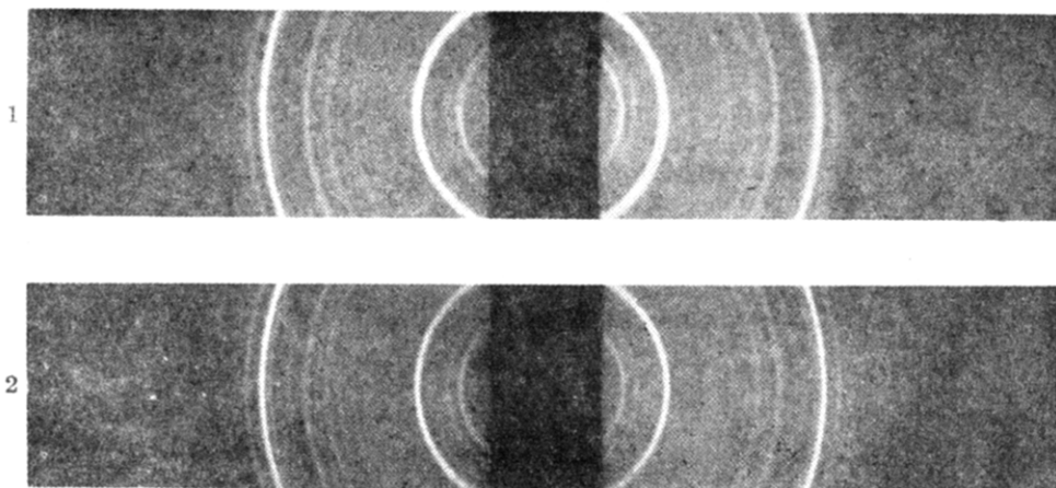
Fig. 4.—X-Ray diffraction patterns of trinitrobenzotates of 1-methyl-5- n -propylnaphthalene: 1, isolated; 2, synthesized.
