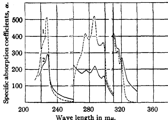
Fig. 3.—Ultraviolet absorption spectra: 1, the hydrocarbon, 1,5-dimethylnaphthalene; 2, the trinitrobenzolate of the isolated and synthetic 1-methyl-5- n -propylnaphthalene (identical curves for the two materials).
