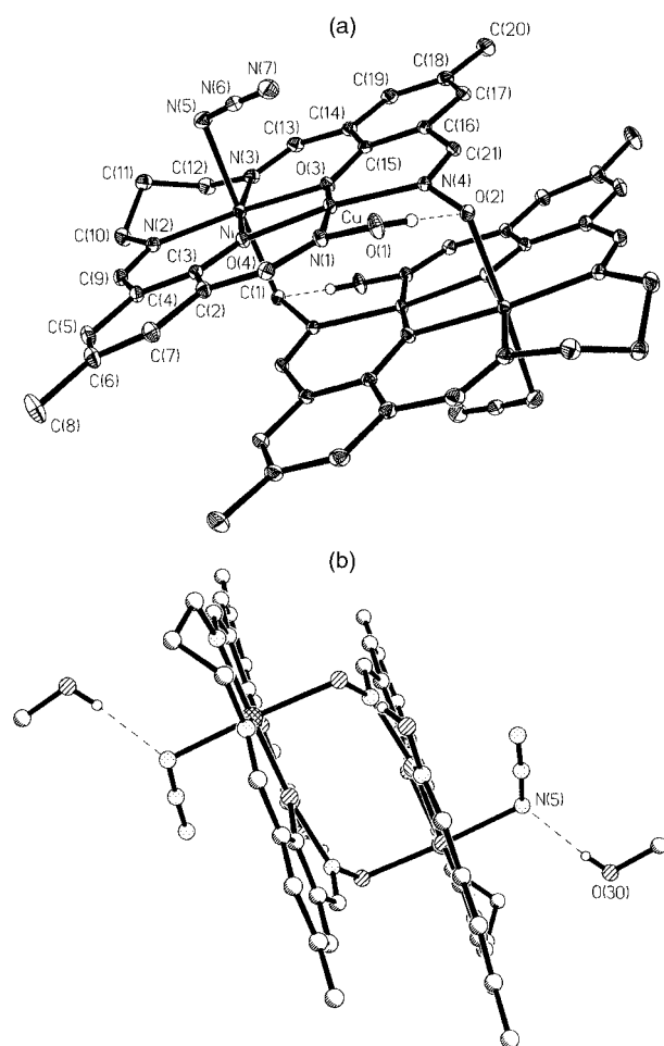
Fig. 1 (a) Molecular structure of [\{\text{Cu}^{\text{II}}(\text{HLOX})\text{Ni}^{\text{II}}(\text{N}_3)\}_2] \mathbf{2} , showing the protonated oximic oxygen. (b) A perspective view of \mathbf{2} highlighting the connectivity between the two \text{Cu}^{\text{II}}\text{Ni}^{\text{II}} units, together with two solvent methanol molecules.
