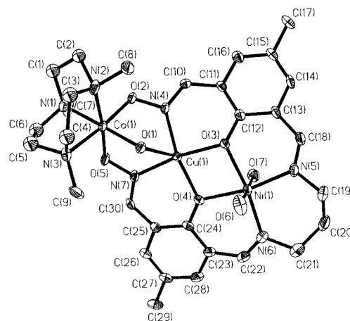
Fig. 2 Structure of the dication containing the \text{Co}^{\text{III}}\text{Cu}^{\text{II}}\text{Ni}^{\text{II}} units in crystals of complex \mathbf{3} .
