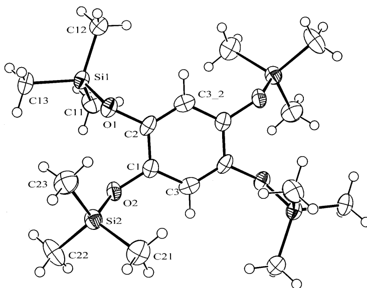
Fig. 2. Molecular structure of 1,2,4,5\text{--}(\text{Me}_3\text{SiO})_4\text{C}_6\text{H}_2 ( 3 ).
