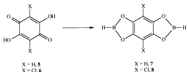
Scheme 2. Syntheses of \text{HBO}_2\text{C}_6\text{X}_2\text{O}_2\text{BH} ( \text{X} = \text{H} , 7 ; \text{X} = \text{Cl} , 8 ). Reagents and conditions: \text{BH}_3\cdot\text{THF} (four equivalents), THF, 12 h at r.t., 40–60%.
