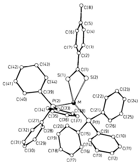
Fig. 3. Perspective view of the complex [M(S_2C\text{-}p\text{-tolyl})(PPh_3)_2] ( M = \text{Au}, \text{Cu} ) (III) with the labelling scheme. Metal site M was 56% Au and 44% Cu.
