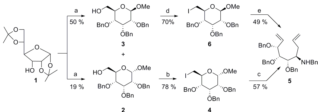
Scheme 1. a) \text{H}_2\text{SO}_4 ; trityl chloride/pyridine/DMAP; DMF; \text{BnBr}/\text{DMF} ; p -TsOH; b) \text{PPh}_3 , imidazole, \text{I}_2 , toluene, 95 °C, 2 h; c) \text{Zn} , THF, 40 °C, ultrasound; \text{BnNH}_2 , 3 h, allyl bromide 4 h; d) \text{PPh}_3 , imidazole, \text{I}_2 , toluene, 95 °C, 2 h; e) \text{Zn} , THF, 40 °C, ultrasound; \text{BnNH}_2 , 3 h, allyl bromide 4 h.
