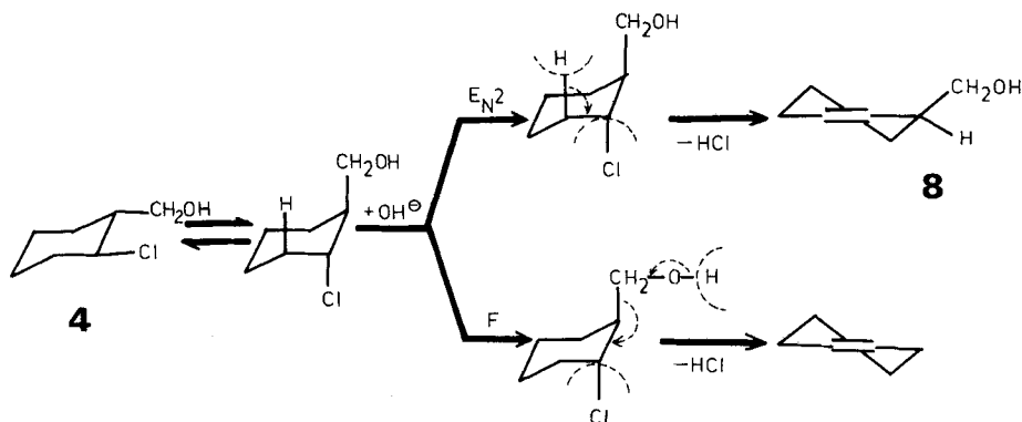
Scheme 5
