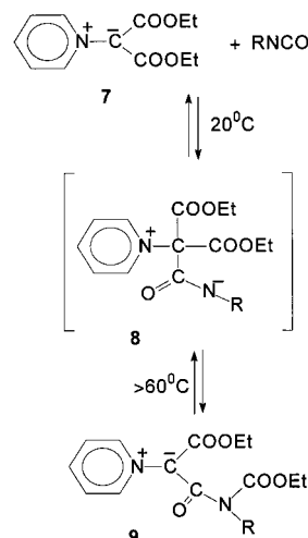
SCHEME 3 R = \text{cyclohexyl} (a), Ph (b), 2-Tolyl (c), 3,4-dichlorophenyl (d), 2-nitrophenyl (e), 4-nitrophenyl (f) and 1-naphthyl (g).
