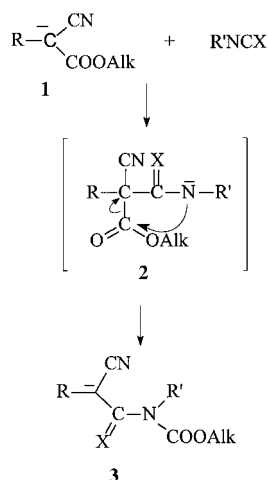
SCHEME 1 R = \text{Pr}_3\text{P}^+\text{CH}_2 , Ph; Alk = Me, Et; X = \text{O} , S; R' = \text{Me} or Ar = Ph, m -Tol, 1-naphthyl, p -ClC 6 H 5 , m,p -Cl 2 C 6 H 3 , C 6 H 5 -NO 2 - p .
