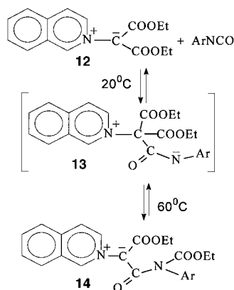
SCHEME 5 Ar = 4- \text{O}_2\text{NC}_6\text{H}_4 (a), 1-naphthyl (b).
