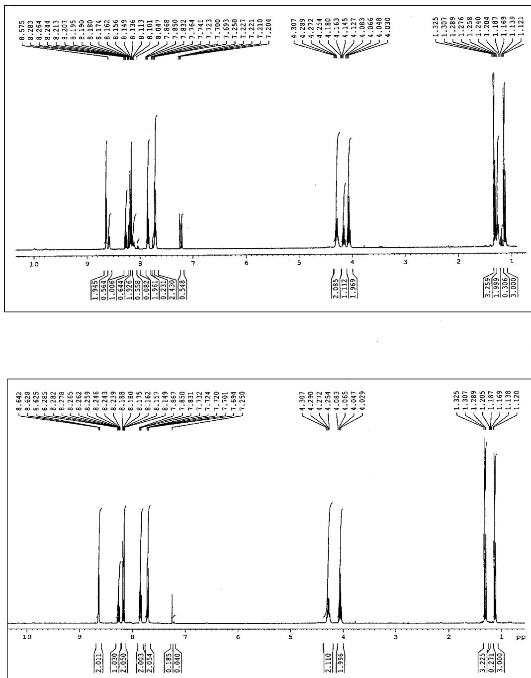
FIGURE 1 ^1\text{H} NMR spectrum of the reaction mixture of ylide 7 (upper picture) and the ylide 9f .
