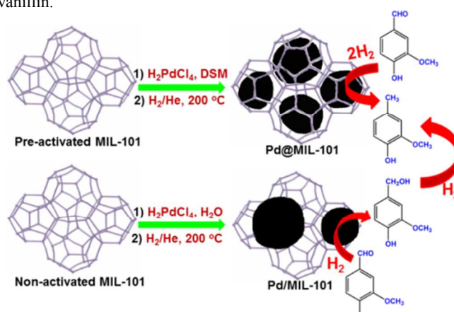
Scheme 1 Schematic representation of the immobilization of Pd nanoparticles into/onto MIL-101, and their use for catalytic hydrodeoxygenation reactions of vanillin.
