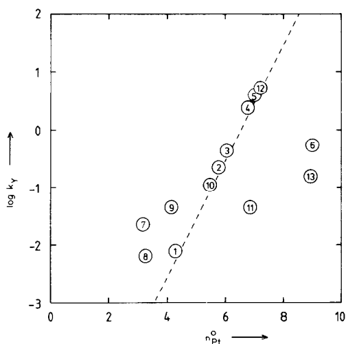
Fig. 2. The dependency \log k_Y = f(n_{\text{Pt}}^0) for solvent substitution in the complex cation [Pt(ONNEt 2 )(H 2 O)] + (the numbering of the nucleophiles Y corresponds to that in Table V).
