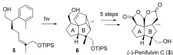
Scheme 1. meta -Photocycloaddition as a Key Step for the Formation of the Carbocyclic Core of the Penifulvins
