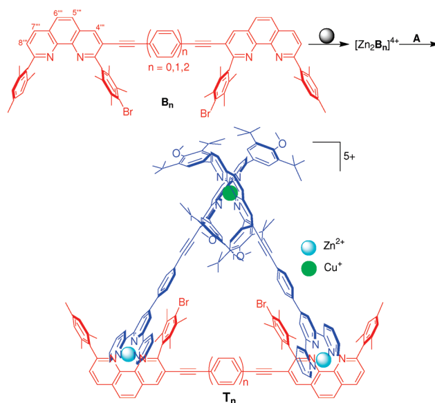
Scheme 2. Self-Assembly of Isosceles Triangles T n
