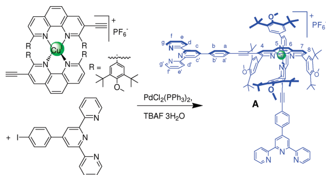
Scheme 1. Synthesis of Angular Complex A
