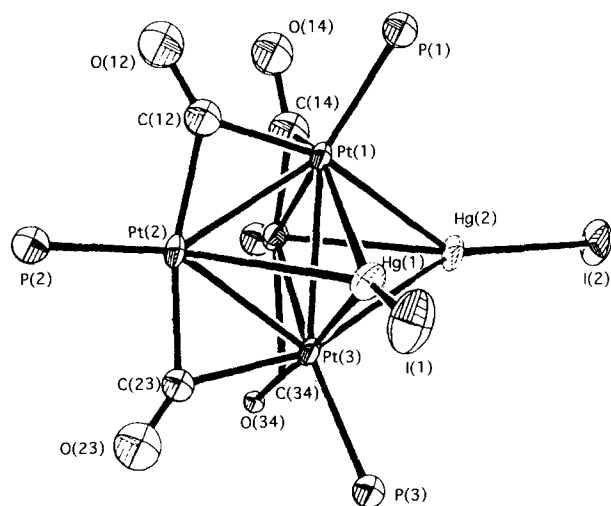
Fig. 1. A view of the structure of [\{\text{Pt}_4(\mu\text{-CO})_4(\text{PMe}_2\text{Ph})_4\}\{\mu_3\text{-HgI}\}_2] (1).
