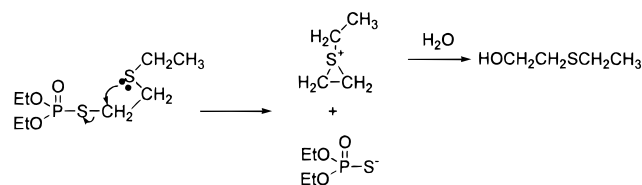
Figure 2. \text{S}_{\text{Ni}} mechanism for demeton-S hydrolysis.
