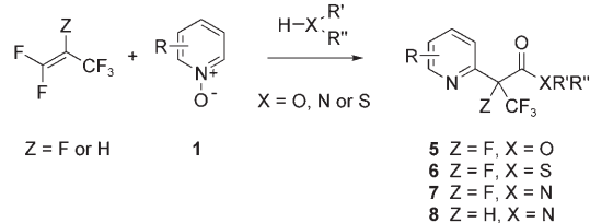
Scheme 3. The novel reaction of azine N -oxides 1 with HFP in the presence of protic nucleophiles presented in this paper.
