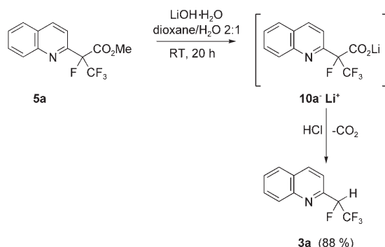
Scheme 8. Hydrolysis of methyl ester 5a leads to the decarboxylated product 3a containing a \text{CHFCF}_3 substituent.
