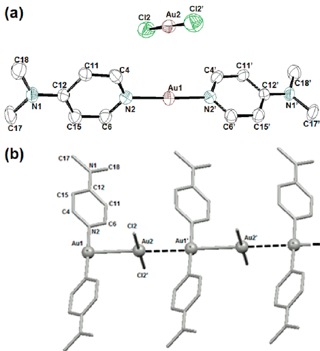
Figure 1. (a) ORTEP diagram of Ia (50% probability ellipsoids), (b) crystal packing diagram of Ia with a [+ - + - \cdots] pattern (the hydrogen atoms have been omitted for clarity). Selected bond lengths (Å) and angles (deg): Au(1)–Au(2), 3.2005(5); Au(1)–N(2), 2.022(3); N(2)–C(6), 1.345(5); N(2)–C(4), 1.348(6); N(1)–C(12), 1.357(5); Au(2)–Cl(2), 2.2659(16); N(2)–Au(1)–N(2'), 177.7(2); C(4)–N(2)–C(6), 116.3(4); Cl(2)–Au(2)–Cl(2'), 179.73(7); Au(1)–Au(2)–Au(1), 180.0.
