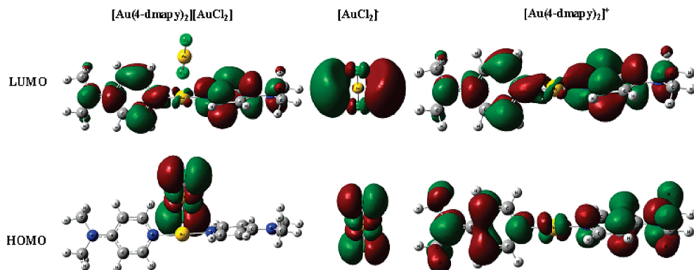
Figure 8. B3LYP/LanL2DZ molecular orbitals of the Ia ion pair, [\text{AuCl}_2]^- , and [\text{Au}(\text{4-dmapy})_2]^+ .
