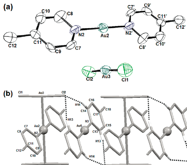
Figure 3. (a) ORTEP diagram of Ila (50% probability ellipsoids), (b) crystal packing diagram of Ila with a [-+ -] [+] pattern (the hydrogen atoms have been omitted for clarity). Selected bond lengths (Å) and angles (deg): Au(2)–Au(3), 3.245(66); Au(2)–N(2), 2.068(48); Au(5)–N(3), 2.066(46); Au(3)–Cl(1), 2.282(12); Au(3)–Cl(2), 2.298(13); N(2)–C(7), 1.350(48); N(2)–C(8), 1.337(53); N(3)–C(13), 1.311(49); N(3)–C(14), 1.351(4); N(2)–Au(2)–N(2'), 180.00(9); N(3)–Au(5)–N(3'), 179.99(1); Cl(1)–Au(3)–Cl(2), 177.42(4); C(7)–N(2)–C(8), 117.72(2); C(13)–N(3)–C(14), 118.64(3).
