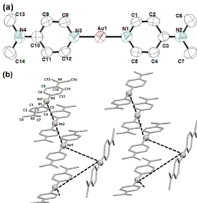
Figure 2. (a) ORTEP diagram of Ib (50% probability ellipsoids), (b) crystal packing diagram of [\text{Au}(\text{4-dmipy})_2]^+ with a [+++] pattern (the [\text{PF}_6]^- ion and hydrogen atoms have been omitted for clarity). Selected bond lengths (Å) and angles (deg): Au(1)–N(1), 2.007(5); Au(1)–N(3), 2.012(5); N(1)–C(1), 1.336(7); N(1)–C(5), 1.354(7); N(3)–C(8), 1.348(7); N(3)–C(12), 1.340(7); N(2)–C(3), 1.349(7); N(4)–C(10), 1.329(7); N(1)–Au(1)–N(3), 177.10(17).
