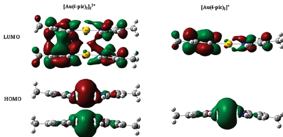
Figure 9. B3LYP/LanL2DZ molecular orbitals of [(\text{Au}(\text{4-pic})_2)_2]^{2+} and [\text{Au}(\text{4-pic})_2]^+ .
