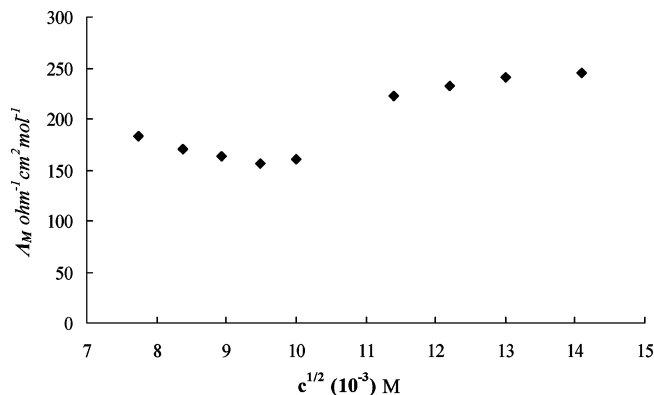
Figure 5. Molar conductivity of a \text{CH}_3\text{CN} solution of IIb , as a function of the square root of the concentration.
