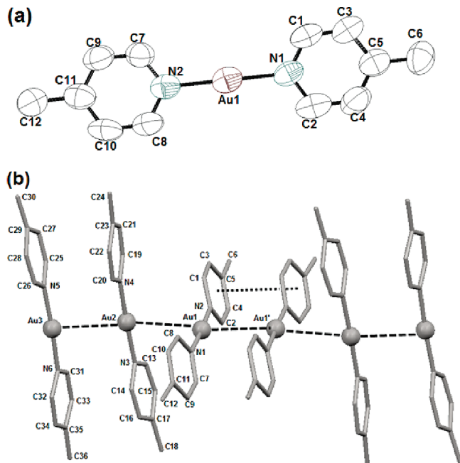
Figure 4. (a) ORTEP diagram of IIb (50% probability ellipsoids), (b) crystal packing diagram of [\text{Au}(\text{4-pic})_2]^+ with a [+++++] pattern (the [\text{PF}_6]^- ion and hydrogen atoms have been omitted for clarity). Selected bond lengths (Å) and angles (deg): (Au(1)–Au(2), 3.2897(6); Au(1)–Au(1') 3.3463(9); Au(2)–Au(3), 3.3242(6); Au(1)–N(1), 2.011(11); Au(1)–N(2), 2.016(11); N(1)–C(1), 1.357(17); N(1)–C(2), 1.336(17); N(2)–C(7), 1.334(16); N(2)–C(8), 1.340(16); N(1)–Au(1)–N(2), 177.8(3); C(1)–N(1)–C(2), 117.6(13); C(8)–N(2)–C(7), 116.7(12); Au(2)–Au(1)–Au(1'), 166.47(3); Au(1)–Au(2)–Au(3), 166.42(2).
